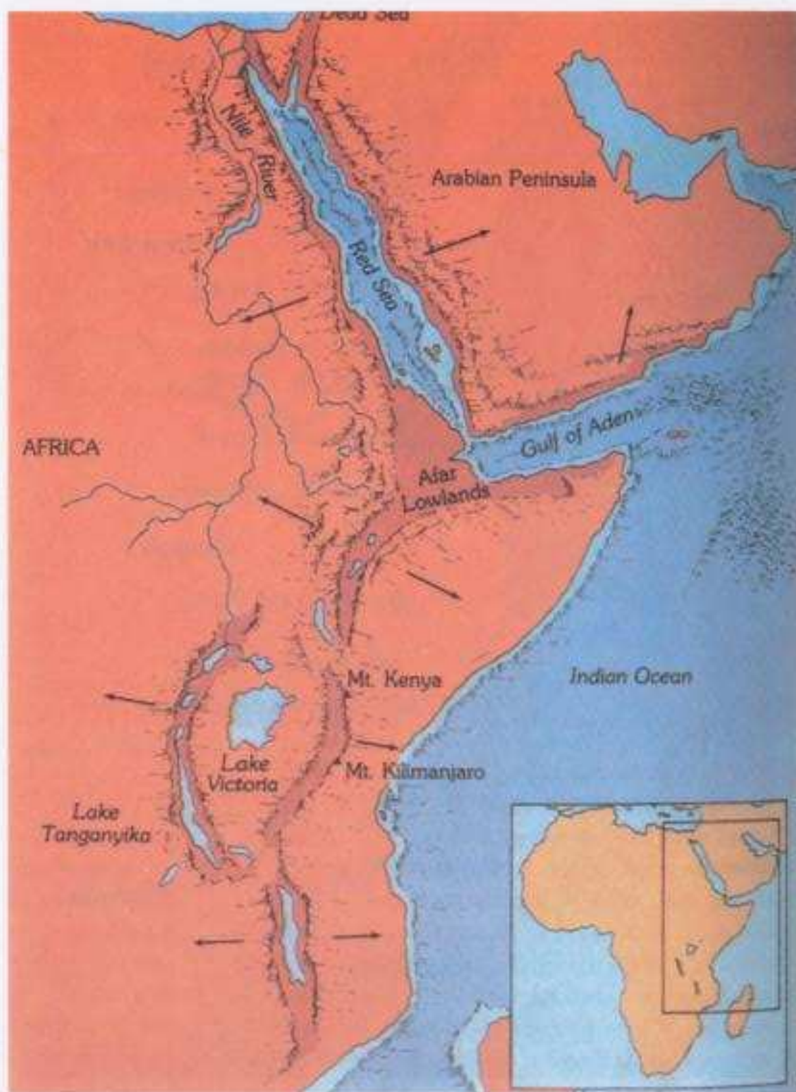
Text-Fig. 14: East African rift valleys and associated features, After Dott & Batten, 1988).
